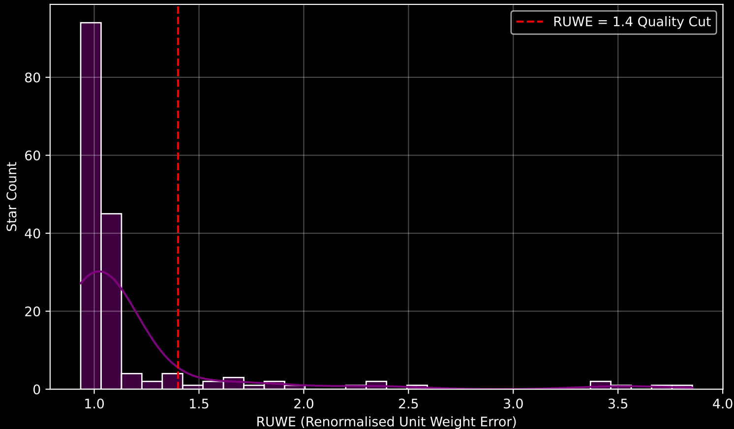
GAPOGEE DR17 Field [SA57-W] RUWE Distribution (n= 168)
