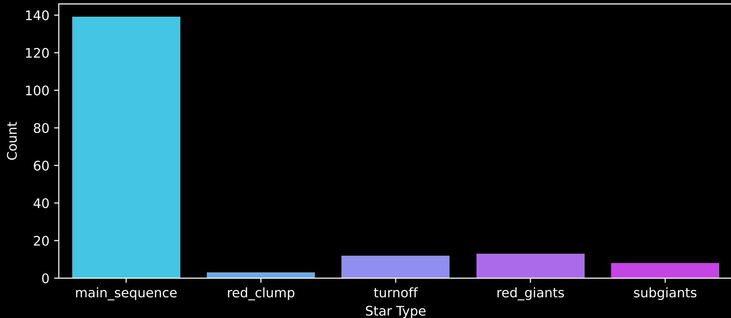
APOGEE DR17 Field: [SA57-W] Count plot of Star Type
