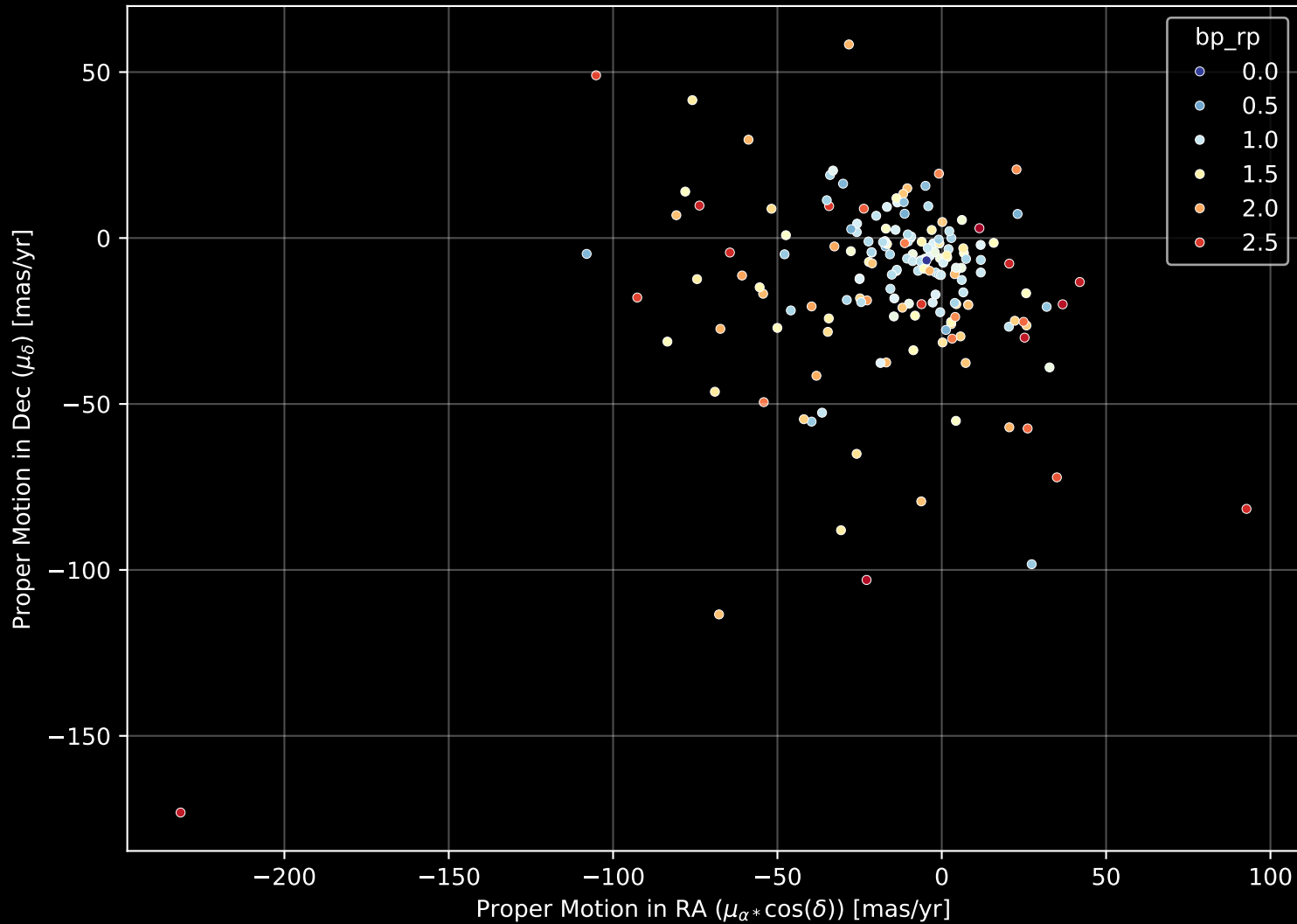
APOGEE DR17 Field: [SA57-W] Proper Motion Diagram (n= 175)
