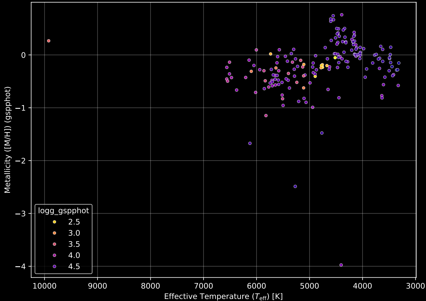
APOGEE DR17 Field: [SA57-W] Stellar Population Parameters (n= 175)
