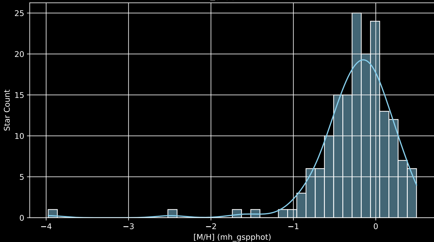
APOGEE DR17 Field: [SA57-W [M/H] (mh_gspphot) (n= 168)
