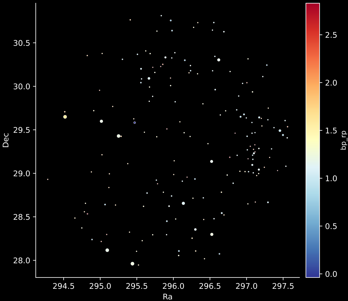
APOGEE DR17 Field: [SA57-W] Stars: 175
