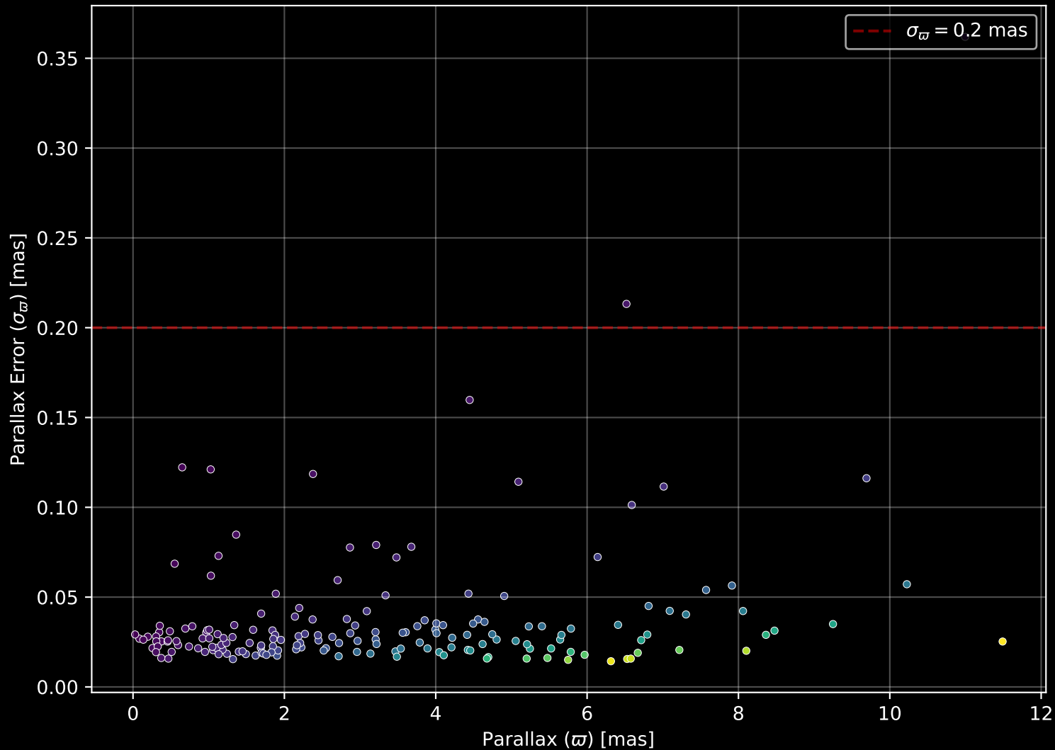
APOGEE DR17 Field: [SA57-W] Parallax Quality (n= 175)
